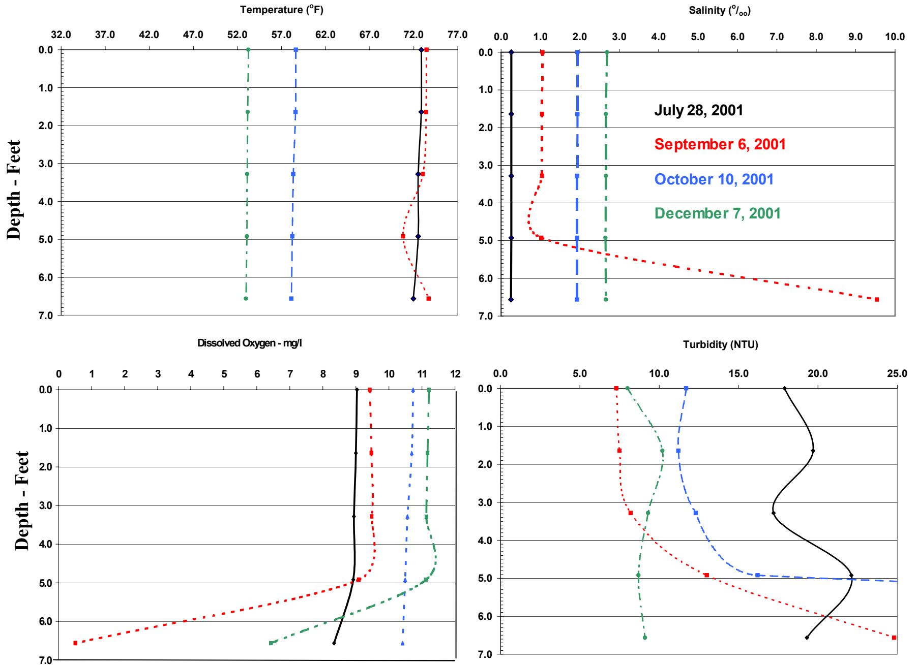
Seasonal profiles of temperature, salinity, dissolved oxygen, and turbidity in Rushy Marsh Pond.
